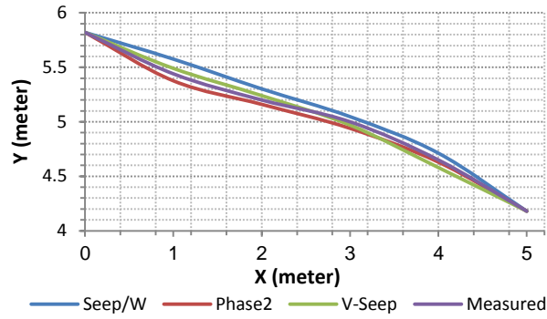
Fig.15. Phreatic Line Diagram
