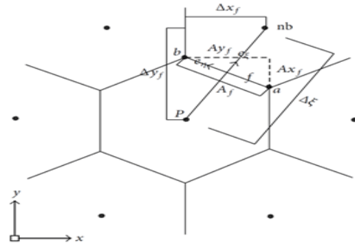
Fig.1. The 2D schematic Voronoi mesh cell used for describing the discretization of the governing equations
