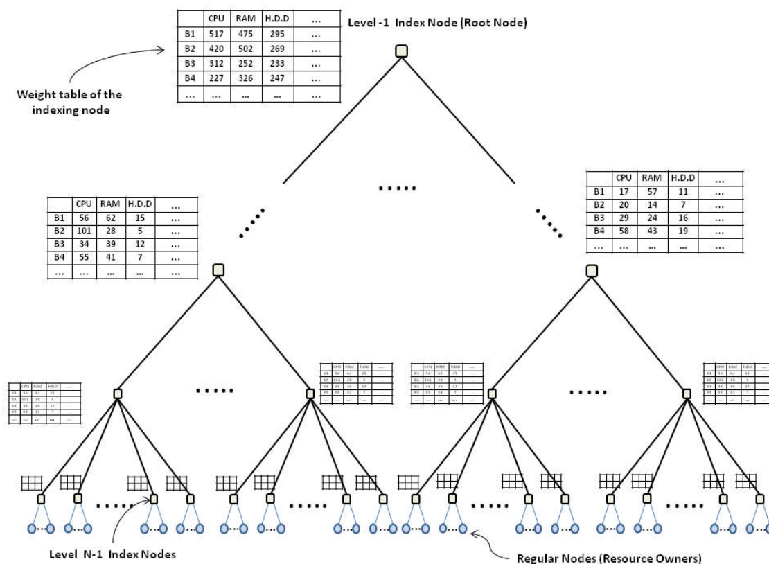
Fig. 1. The indexing schema of weighted-hr resource discovery technique.
