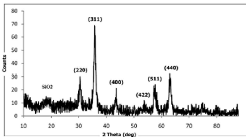
Figure 6. XRD pattern of the MNP-TA catalyst.
