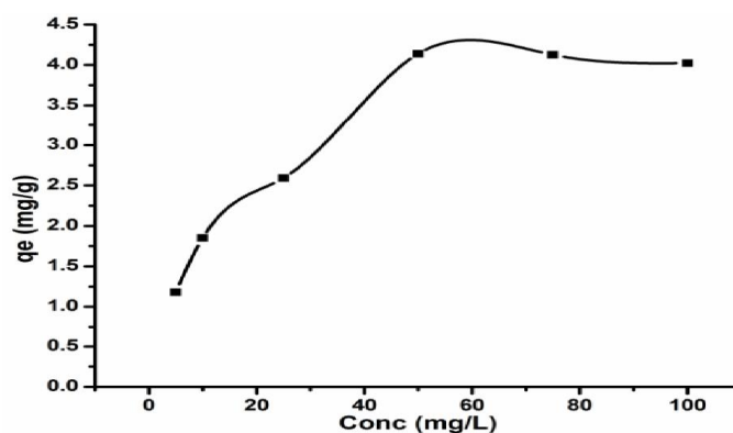
Figure 5. Effect of initial concentration on the sorption of BPA onto RHS (pH 7; 60 min; 0.2 g of RHS; at 303K).
