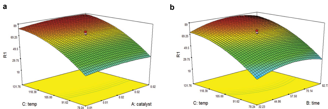
Fig. 5. (a) 3D plot of the response surface of Biginelli reaction (57 min). (b) 3D plot of the response surface of Biginelli reaction (0.016 g).
