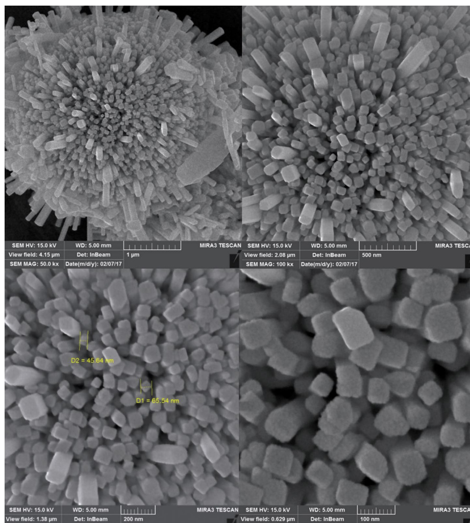
Fig. 2. FESEM images of the hydrothermally synthesized \text{CuBi}_2\text{O}_4 nanomaterials.
