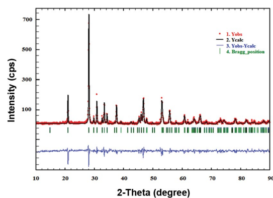
Fig. 1. calculated PXRD pattern for Rietveld profile of synthesized CuBi 2 O 4 .
