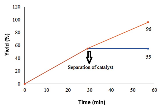
Fig. 6. Hot filtration test of the catalyst under free solvent condition.
