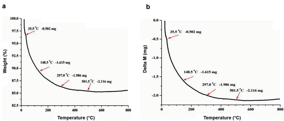
Fig. 3. (a) TGA pattern of \text{CuBi}_2\text{O}_4 . (b) DTA pattern of \text{CuBi}_2\text{O}_4 .
