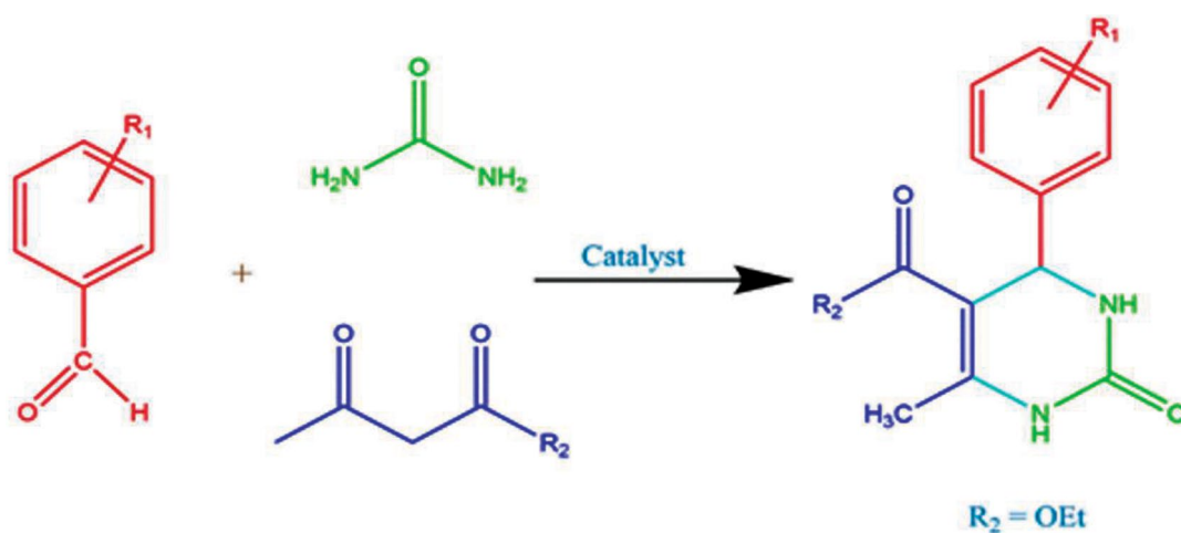
Scheme. 1. Schematic preview for synthesizing DHPMs.
